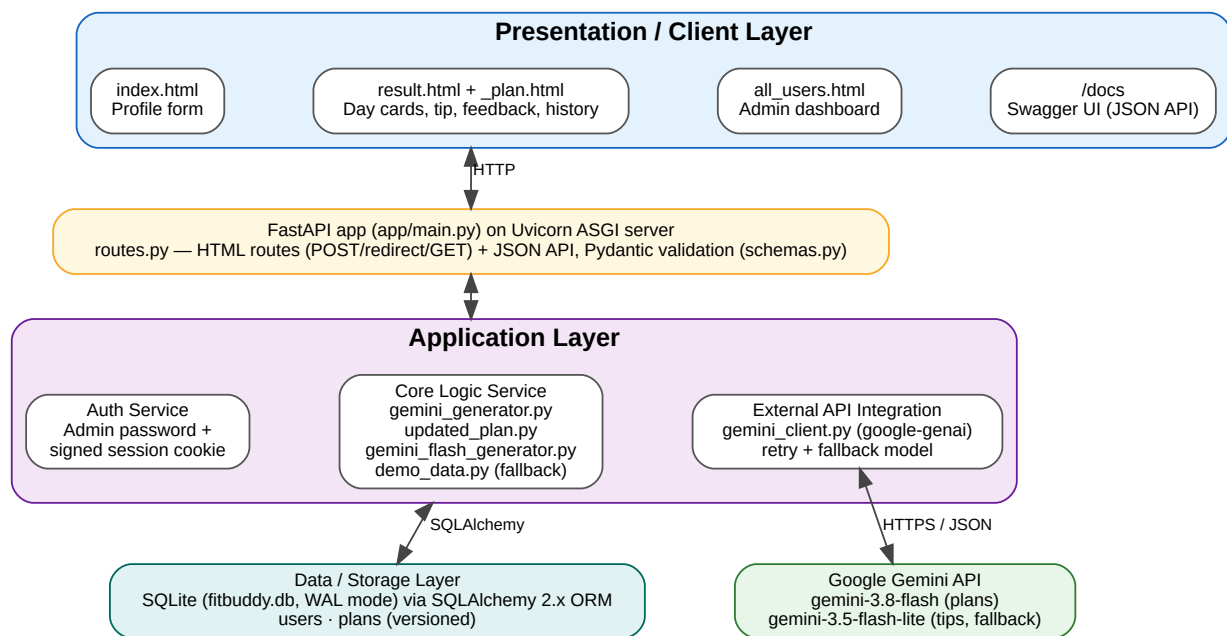
Figure 1: FitBuddy solution architecture
