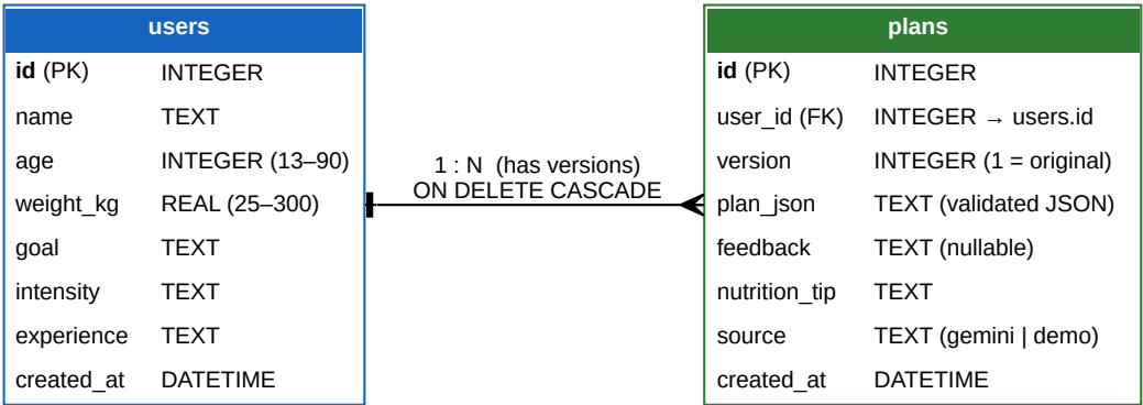
Figure 2: FitBuddy ER diagram — one user has many plan versions
